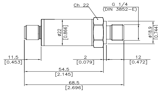
Connector M12x1
