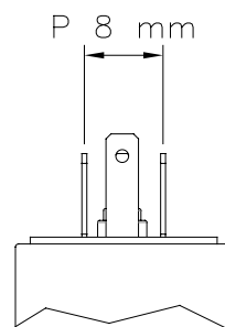
4 pin MicroDIN Form C Protection IP65
