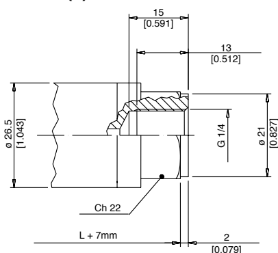
(4) G 1/4 FEMALE
